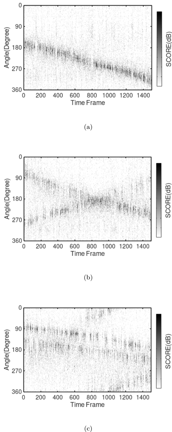
Fig. 12: Potential DOA distribution with mobile sources: (a) One mobile source; (b) Two mobile sources; and (c) Three mobile sources.
